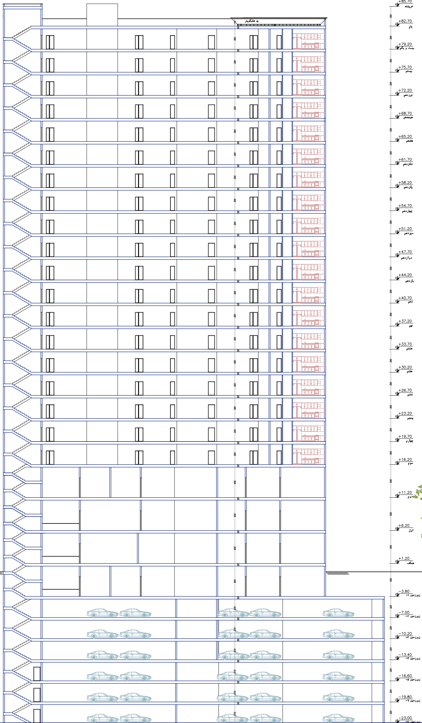
SECTION B-B
